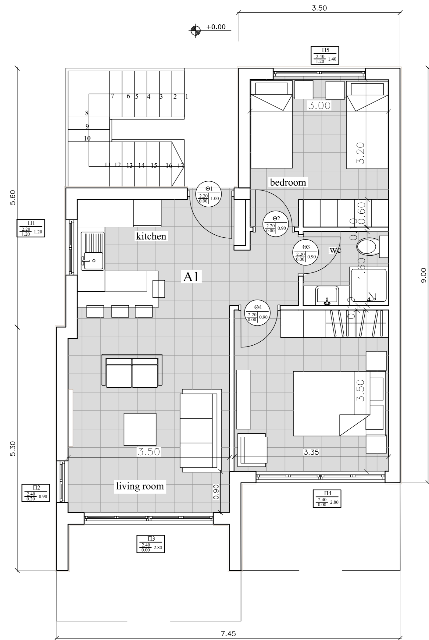
GROUND FLOOR Building A
