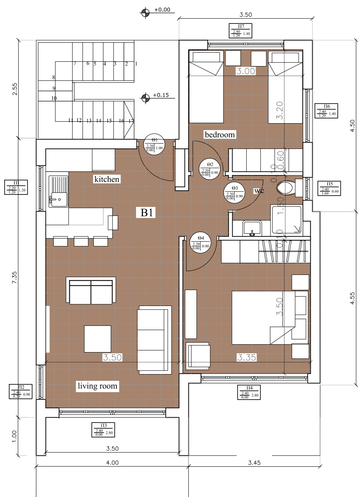
GROUND FLOOR Building B
