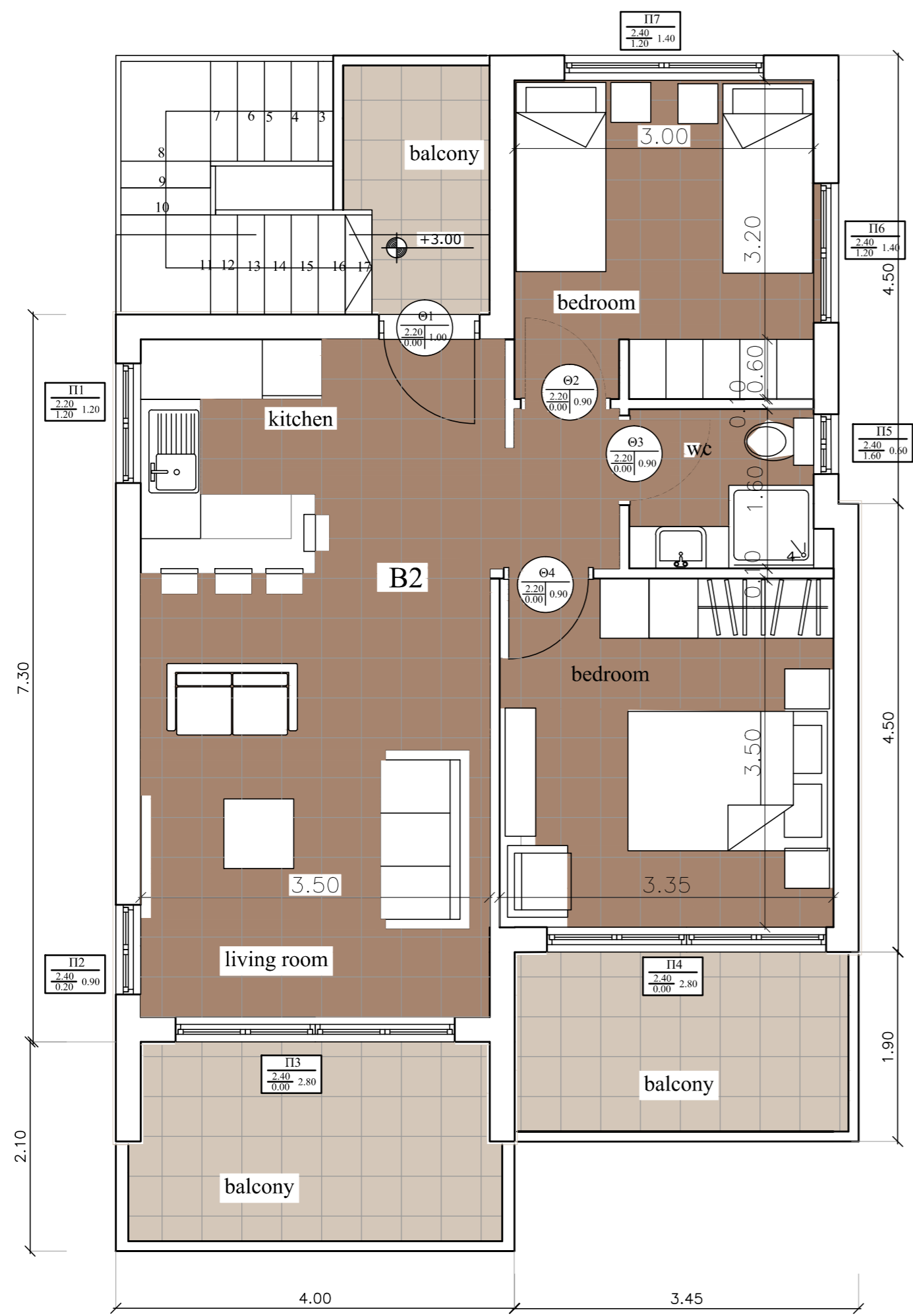
1ST FLOOR Building B
