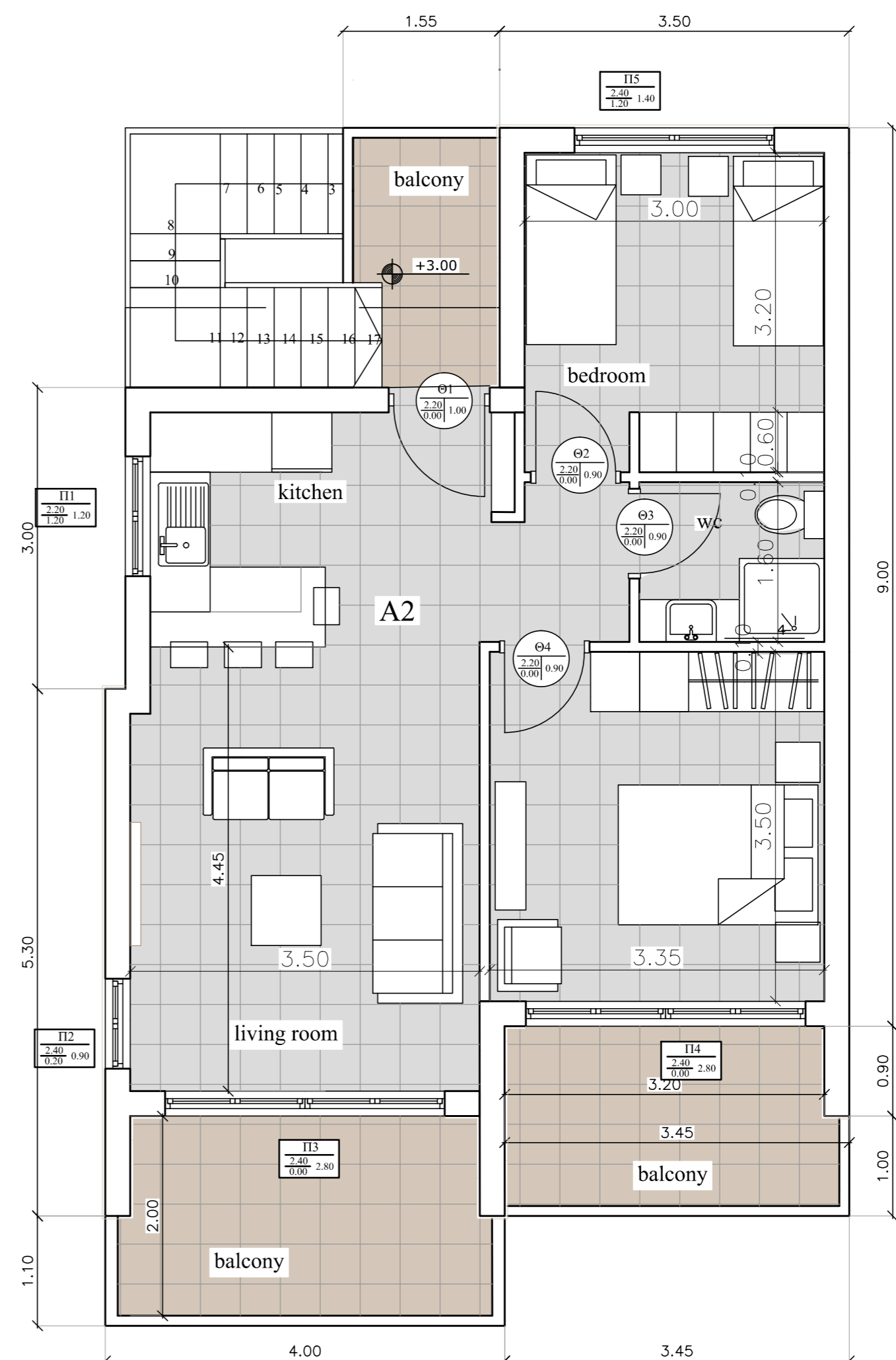
1ST FLOOR Building A
